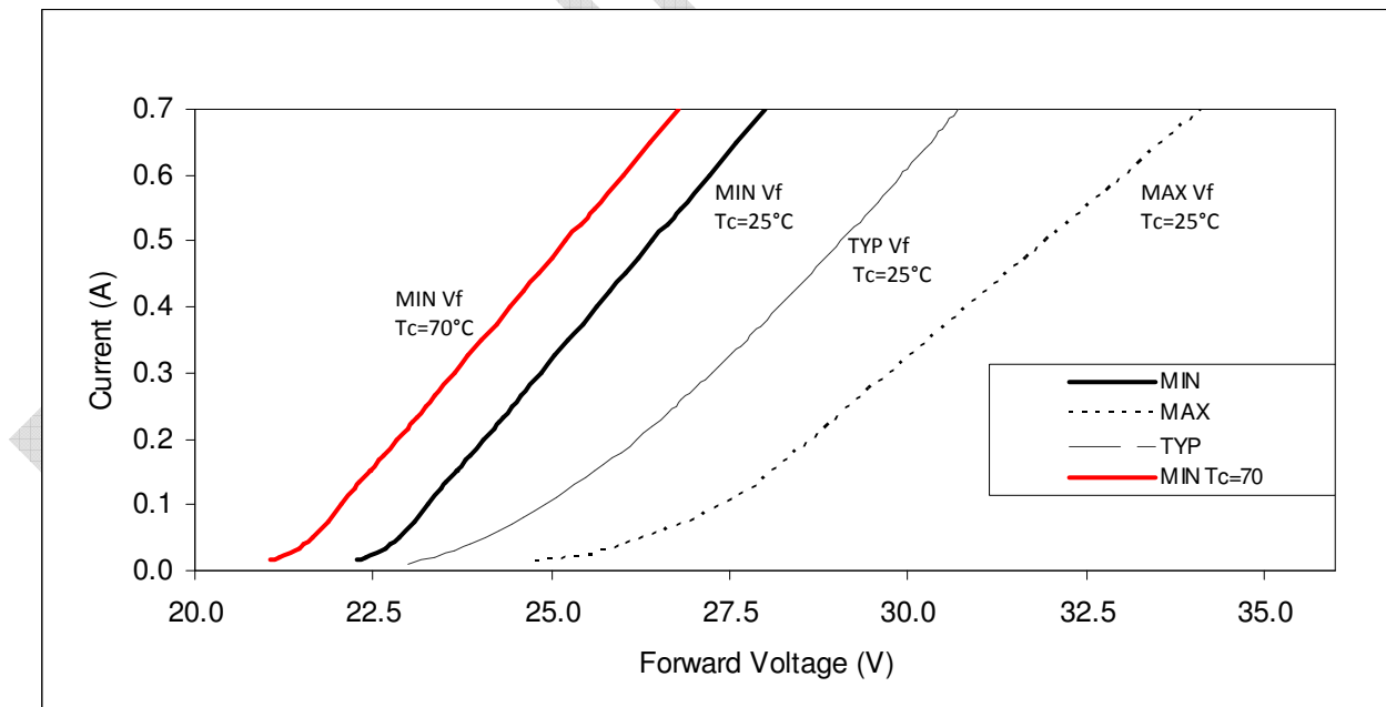
Figure 11: Typical Current vs. Voltage BXRA-xxx0740-A, BXRA-40E0810-A, BXRA-56C1000-A
