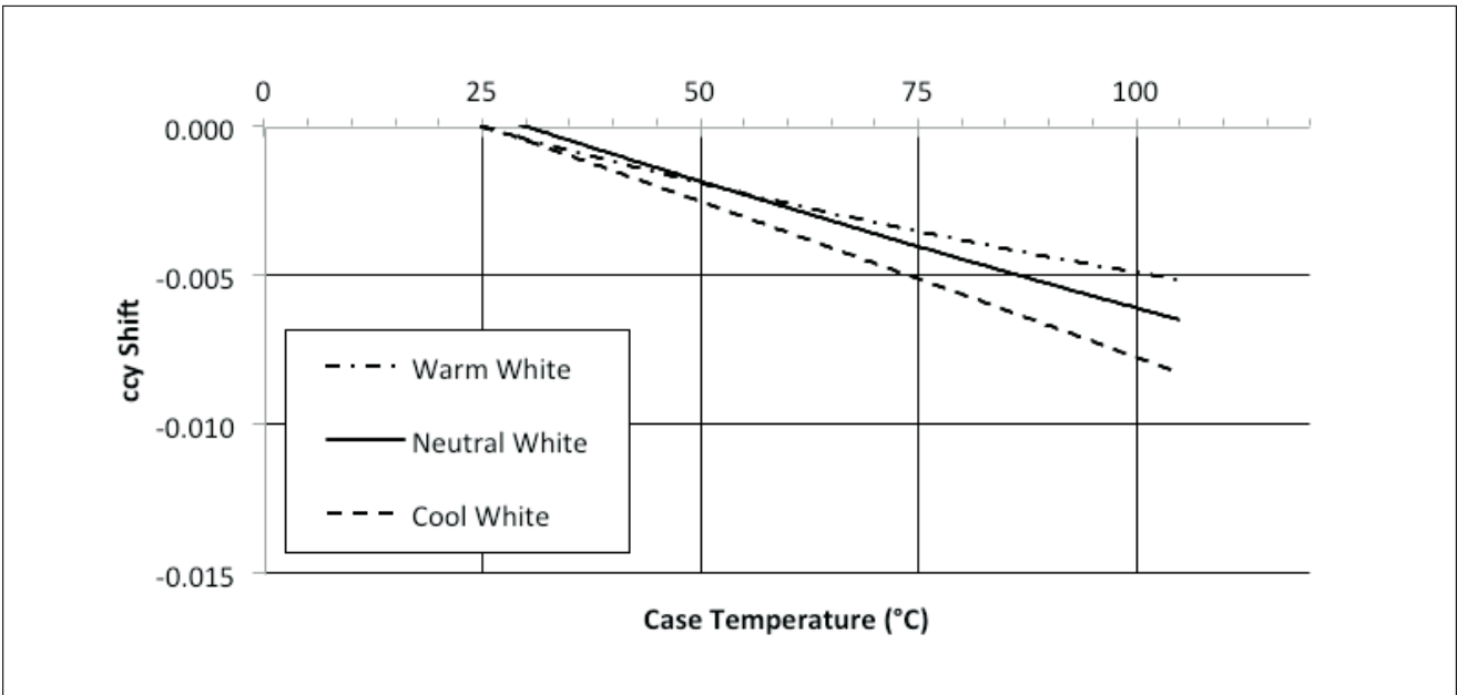
Figure 5: Typical ccy Shift vs. Junction Temperature
