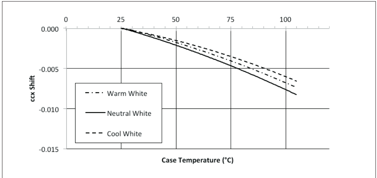
Figure 6: Typical ccx Shift vs. Junction Temperature
