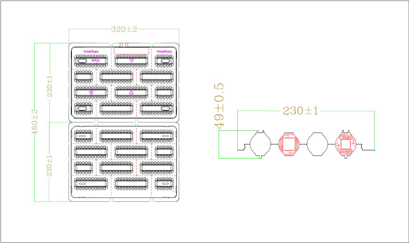
Figure 16: Drawing for Vero SE 18 Packaging Tray
