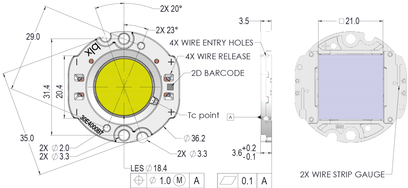
Figure 13: Drawing for Vero SE 18 LED Array
