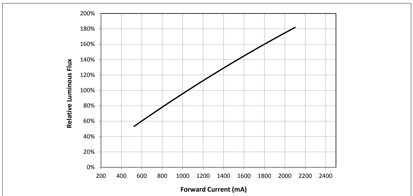
Figure 6 Vero SE 18D Typical Relative Flux vs. Current ( T_j = T_c = 25^\circ\text{C} )
