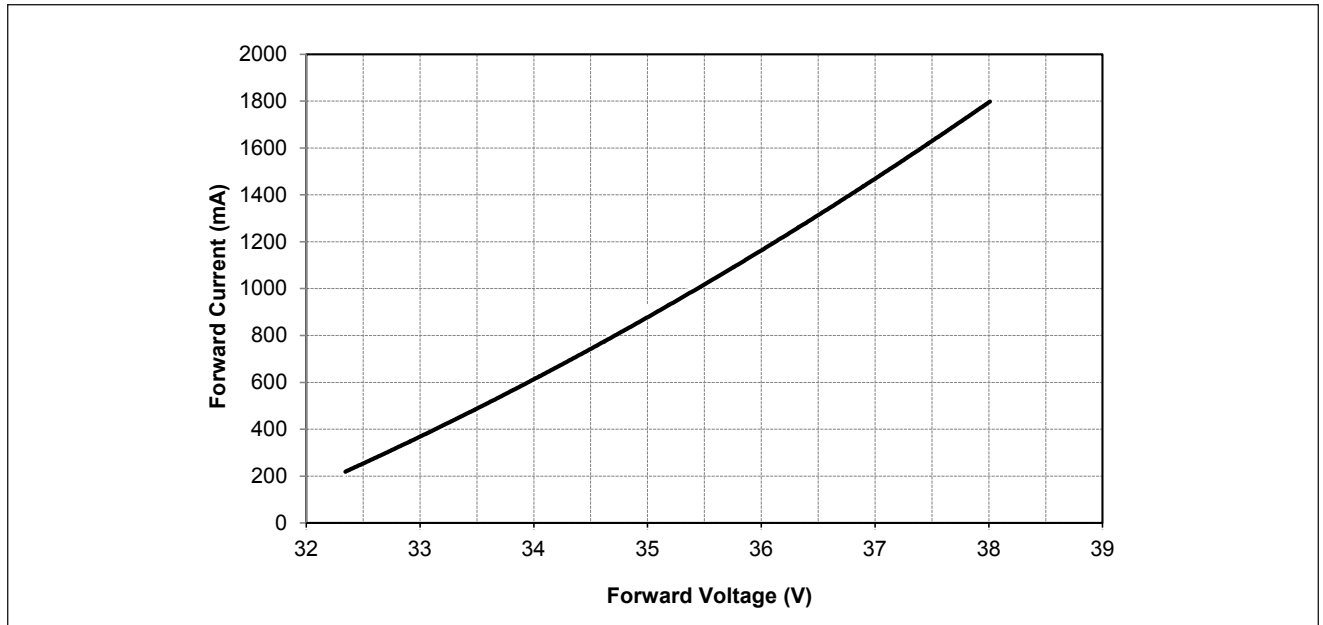
Figure 1: Vero SE 18B Drive Current vs. Voltage ( T_j = T_c = 25^\circ\text{C} )
