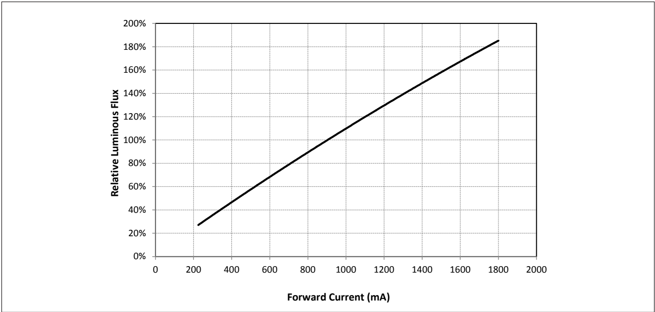
Figure 4: Vero SE 18B Typical Relative Flux vs. Current ( T_j = T_c = 25^{\circ}\text{C} )
