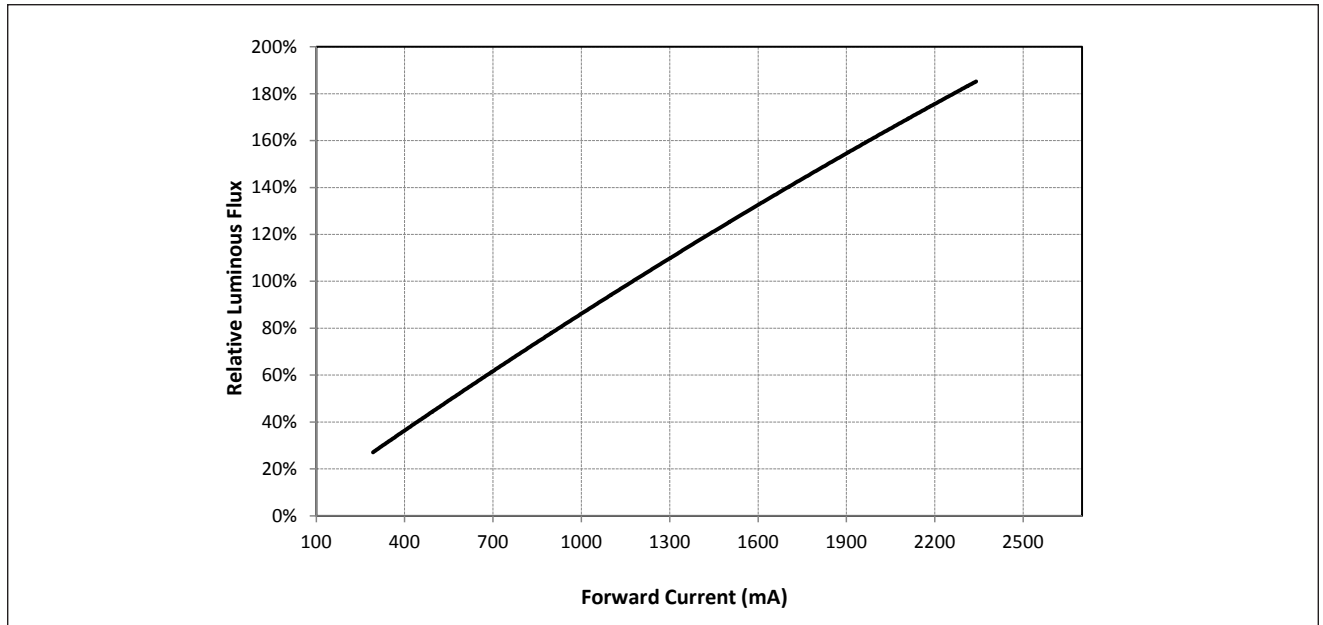
Figure 5: Vero SE 18C Typical Relative Flux vs. Current ( T_j = T_c = 25^\circ\text{C} )
