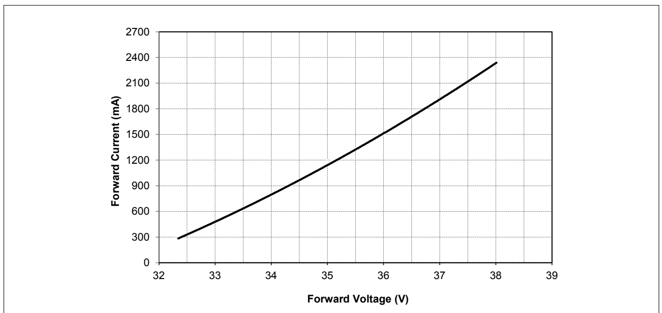
Figure 2: Vero SE 18C Drive Current vs. Voltage ( T_j = T_c = 25^\circ\text{C} )
