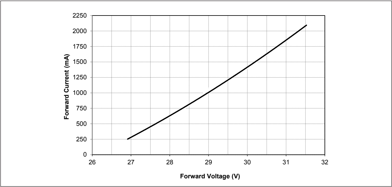
Figure 3: Vero SE 18D Drive Current vs. Voltage ( T_j = T_c = 25^{\circ}\text{C} )
