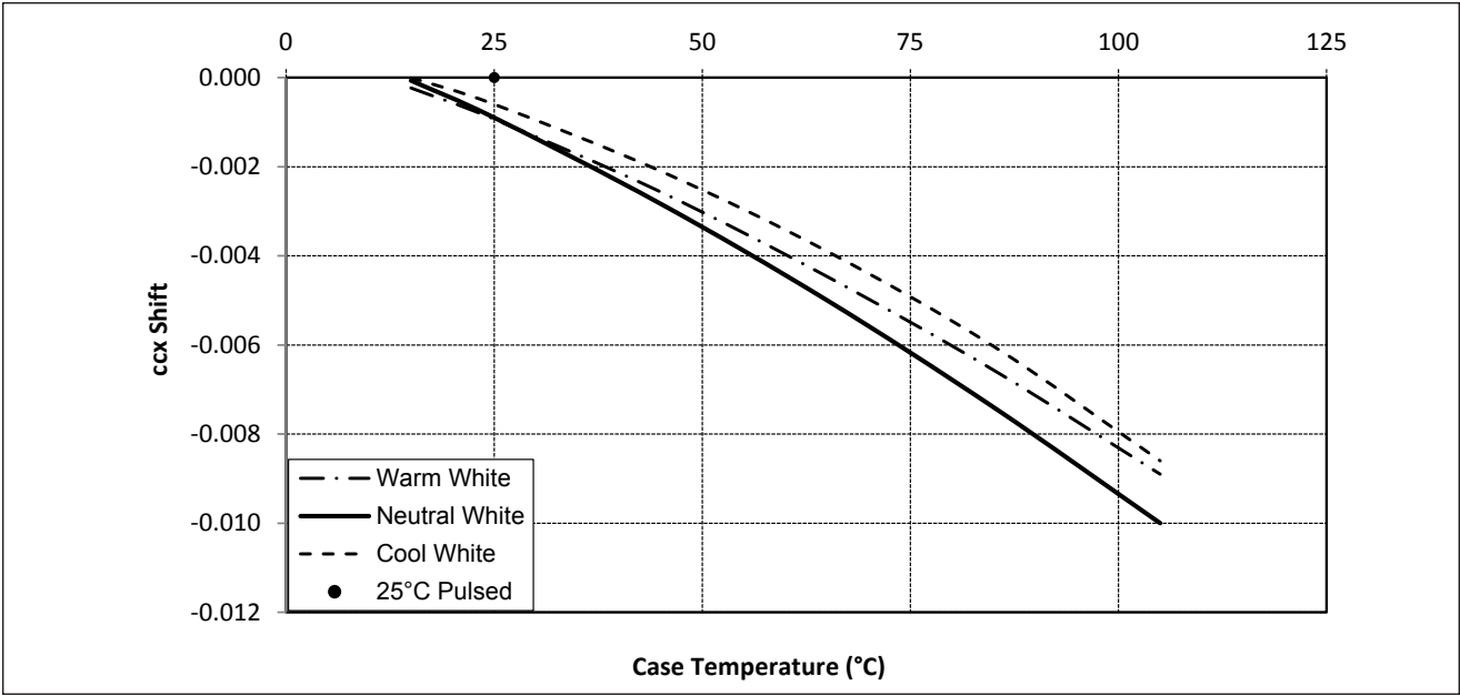
Figure 7: Typical DC ccx Shift vs. Case Temperature
