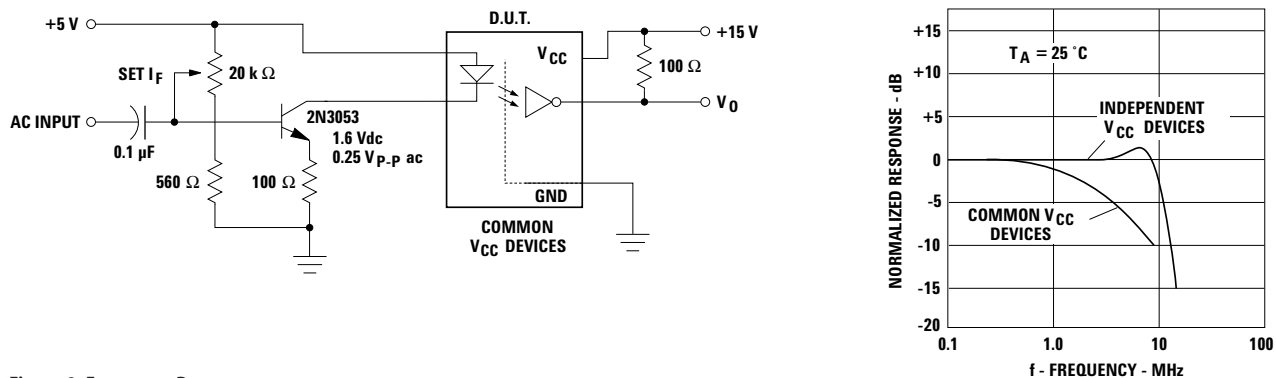
Figure 8. Frequency Response.
