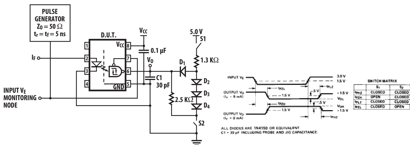
Figure 8. Test circuit for t_{PHZ} , t_{PZH} , t_{PLZ} , and t_{PLZ} (single channel product only)
