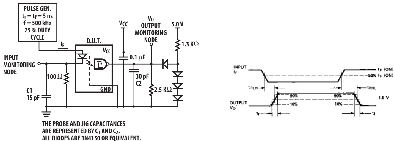
Figure 5. Test circuit for t_{PLH} , t_{PLH} , t_r , and t_f
