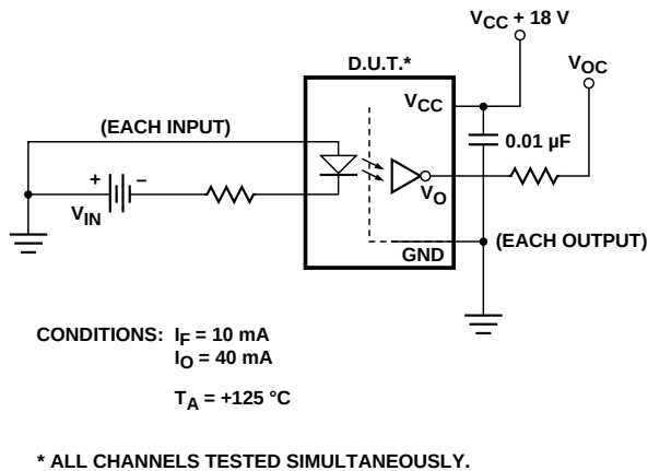
Figure 11. Operating Circuit for Burn-In and Steady State Life Tests.
