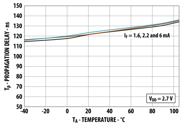
Figure 8. Propagation Delay, t_{PL} vs. Temperature
