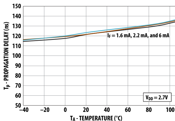
Figure 13 Propagation Delay, t_{pHL} vs. Temperature
