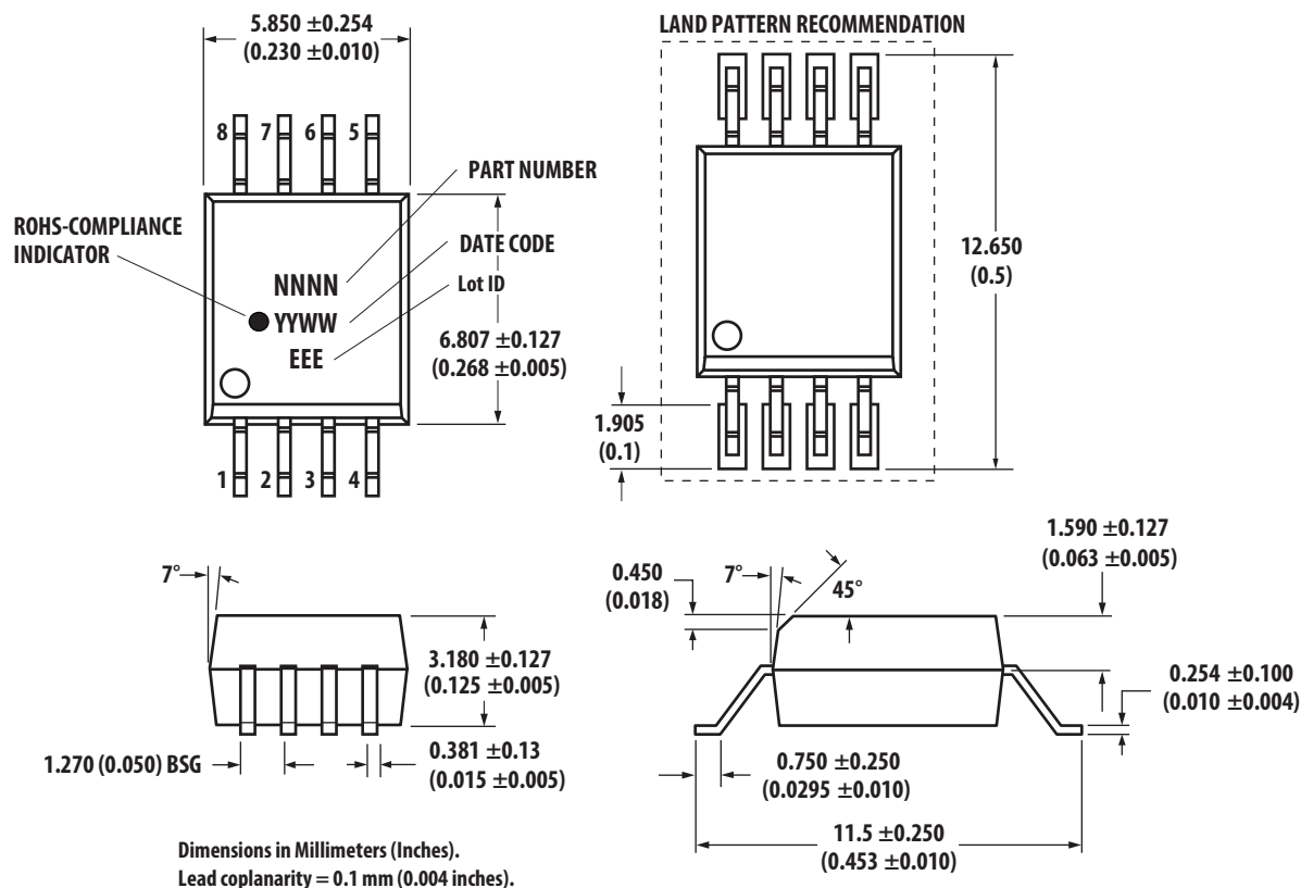
Figure 5 ACPL-K24L Stretched SO-8 Package
