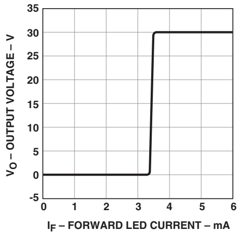
Figure 15. Transfer Characteristics.
