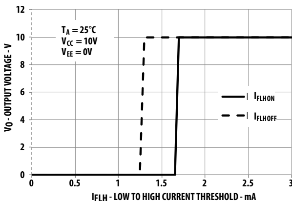
Figure 6: I_{FLH} Hysteresis
