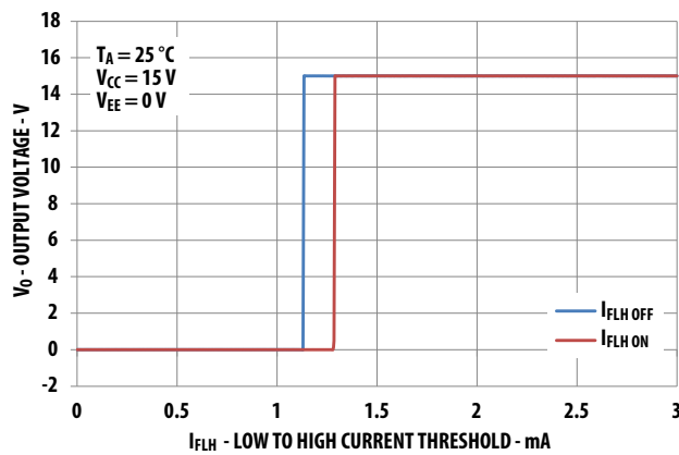
Figure 5. I_{FLH} hysteresis
