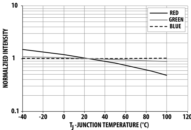
Figure 5. Relative Luminous Flux vs. Junction Temperature
