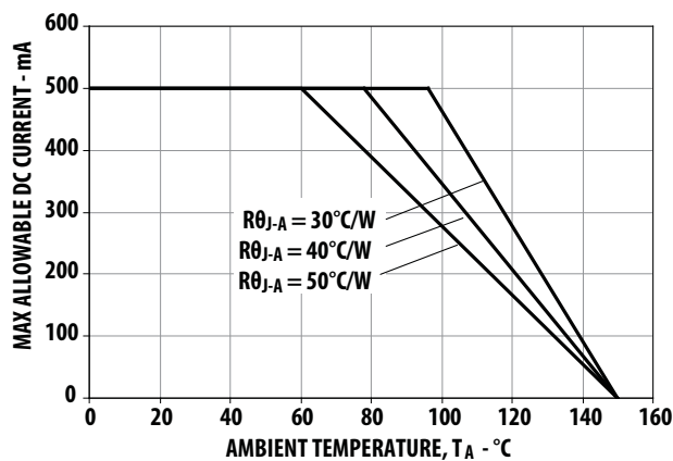
Figure 22. Maximum Forward Current vs. Ambient Temperature. Derated based on T_{JMAX} = 150^\circ\text{C} , R_{\theta JA} = 30^\circ\text{C/W} , 40^\circ\text{C/W} and 50^\circ\text{C/W}
