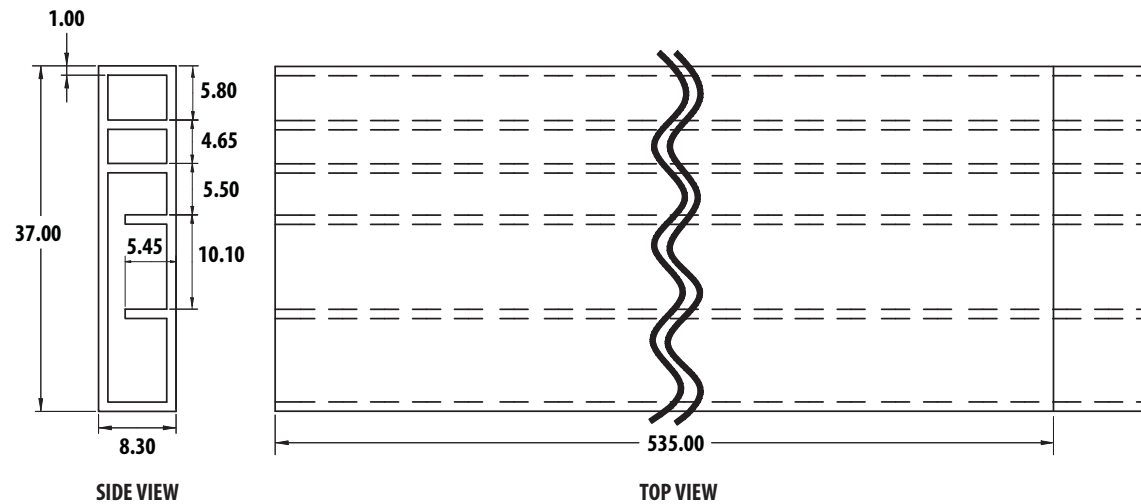
Figure 17. Tube dimensions
