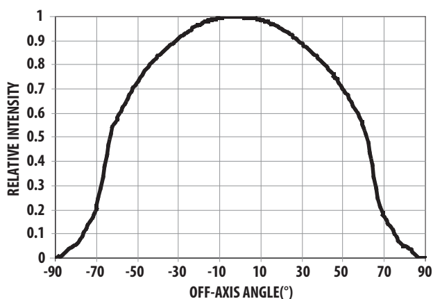
Figure 4. Radiation Pattern for AllnGaP
