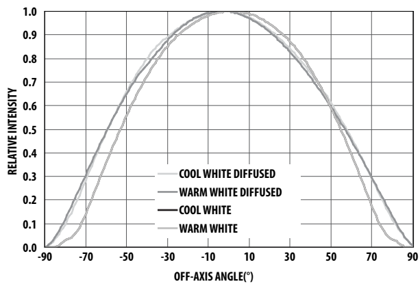
Figure 4. Radiation Pattern
