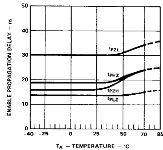
Figure 10. Typical Enable Propagation Delay vs. Ambient Temperature.
