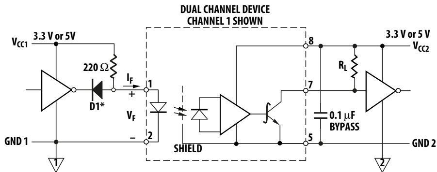
Figure 12. Recommended LVTTL interface circuit
