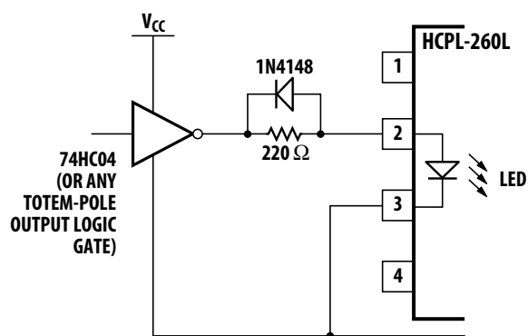
Figure 17. CMOS gate drive circuit
