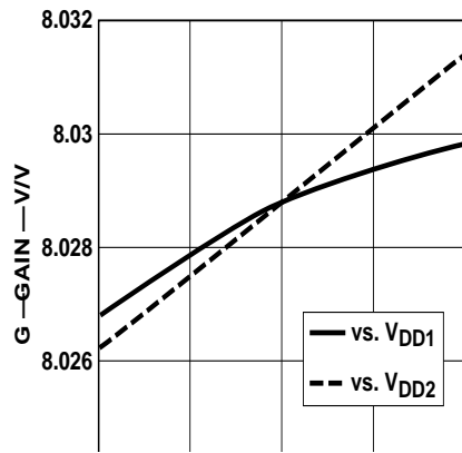
Figure 6. Gain vs. Supply.
