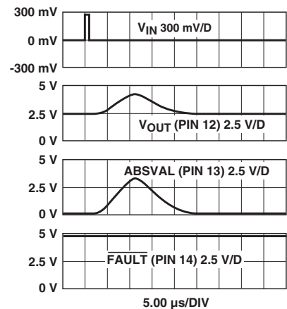
Figure 17. \overline{\text{FAULT}} rejecting a 1 \mu\text{s} , 0 to 2 V to 0 input. Rejection is independent of amplitude.
