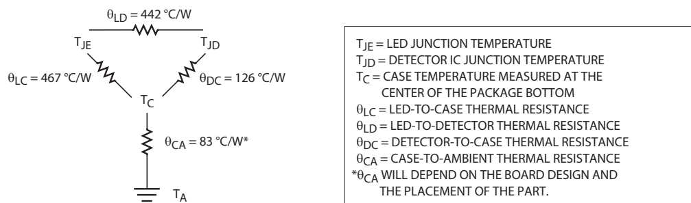
Figure 28 Thermal Model
