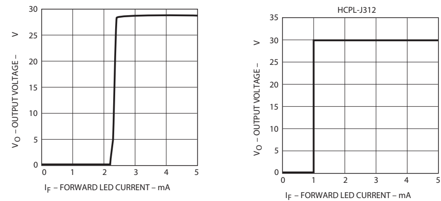
Figure 15 Transfer Characteristics
