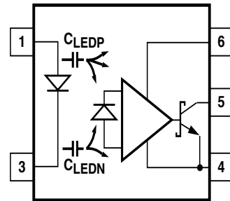
Figure 14. Optocoupler Input to Output Capacitance Model for Unshielded Optocouplers.
