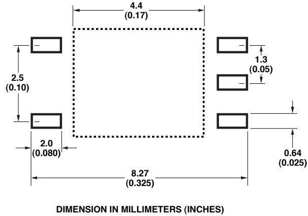
Figure 1.5 5 Pin SOIC Package (JEDEC MO-155) Device Outline Drawing.
