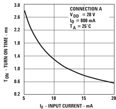
Figure 12. Typical Turn On Time vs. Input Current.
