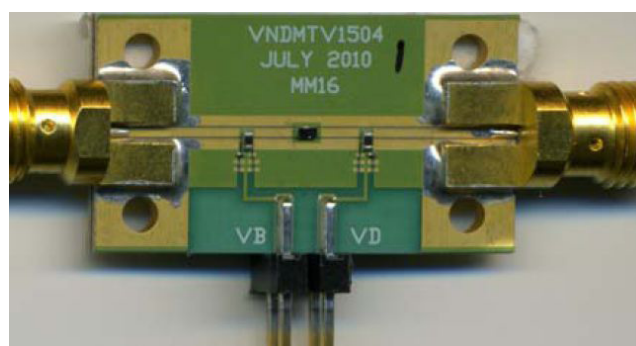
Figure 8. VMMK-3213 Characterization Board (Note: Need two external DC blocking caps)
