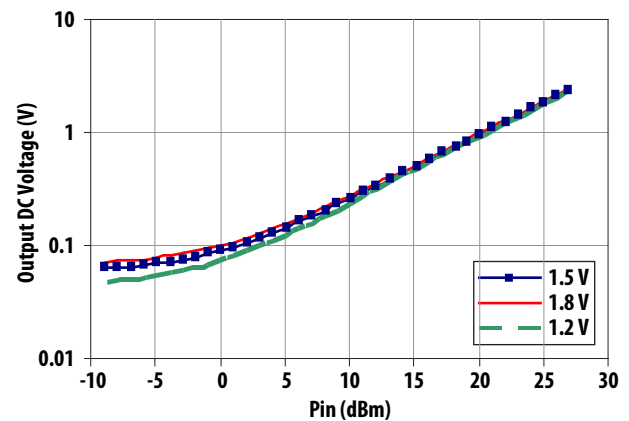
Figure 6. Pin vs. Vdet Over Vbias at 12 GHz
