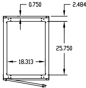
TOP VIEW (LESS TOP COVER & TOP COWLS)
