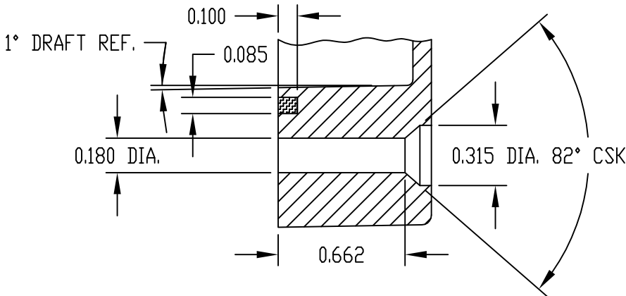
DETAIL "D"
