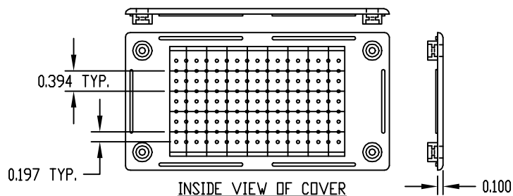
INSIDE VIEW OF COVER
