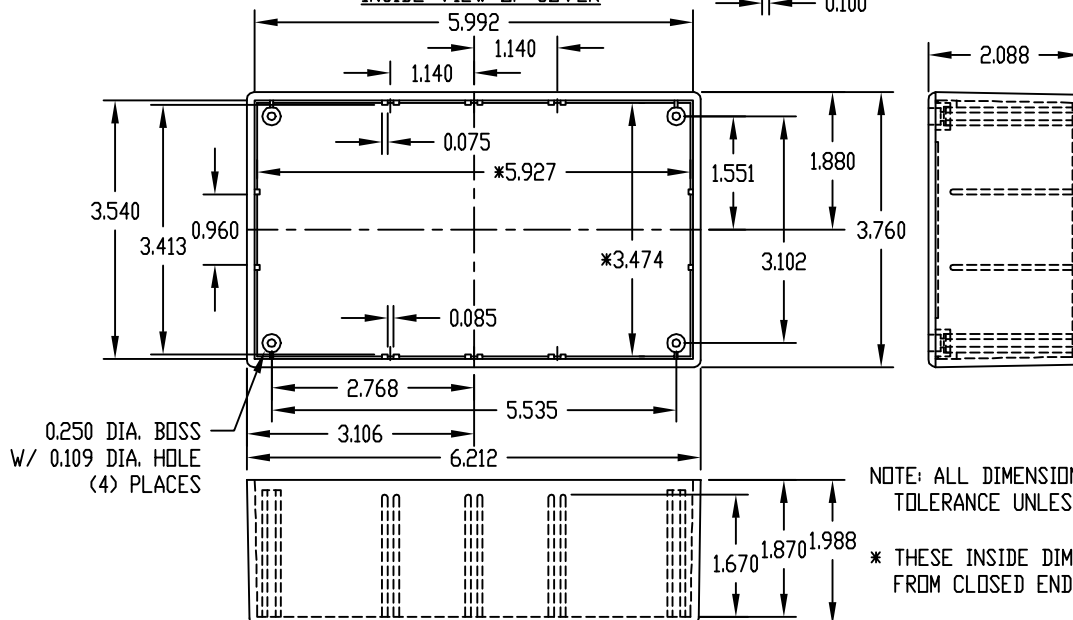
INSIDE VIEW OF COVER
