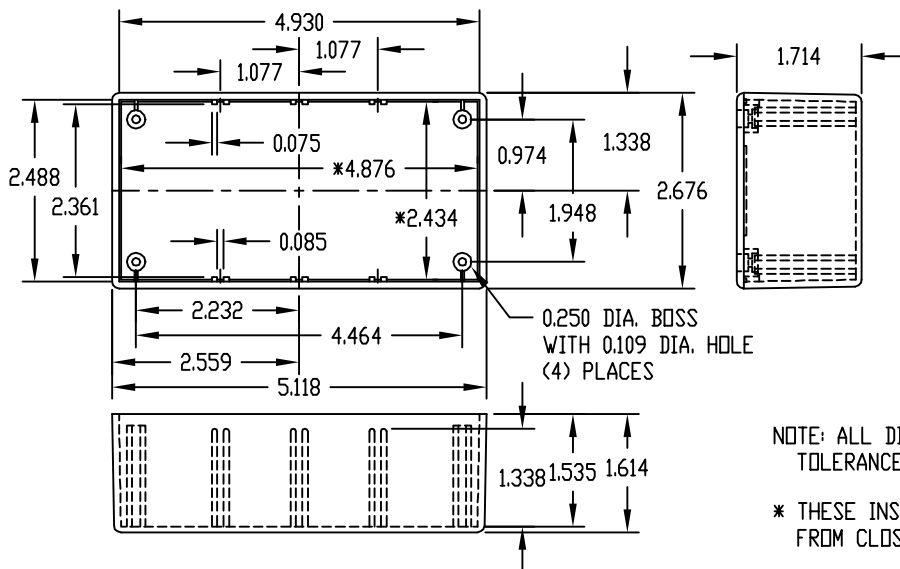
INSIDE VIEW OF COVER
