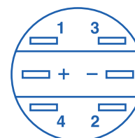
Pin Layout
