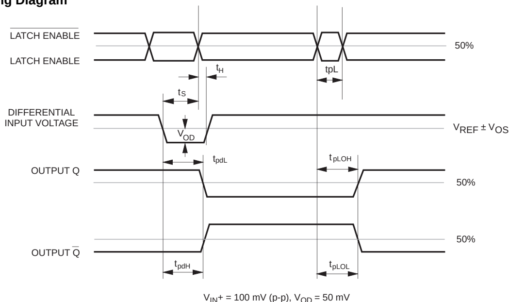
Figure 1 - Timing Diagram
