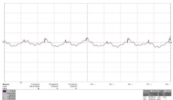
Fig. 27: Input reflected ripple current, i_C (500 mA/mV), measured at input terminals at full rated load current at V_{IN} = 24V . Refer to Fig. 2 for test setup. Time: 2 \mu s/div. RMS input ripple current is 1.205 \times 500mA = 602.5mA .
