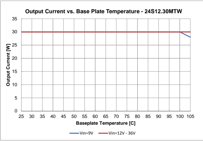
Fig. 11: 24S12.30MTW (ROHS) Derating Curve
