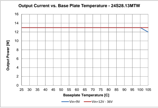
Fig. 15: 24S28.13MTW (ROHS) Derating Curve
