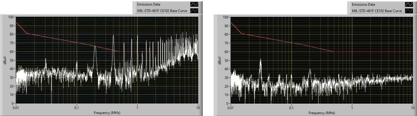
a) Without input filter. C_{IN} = 2 \times 470\mu\text{F}/50\text{V}/70\text{m}\Omega . b) With input filter from Fig. 28.
