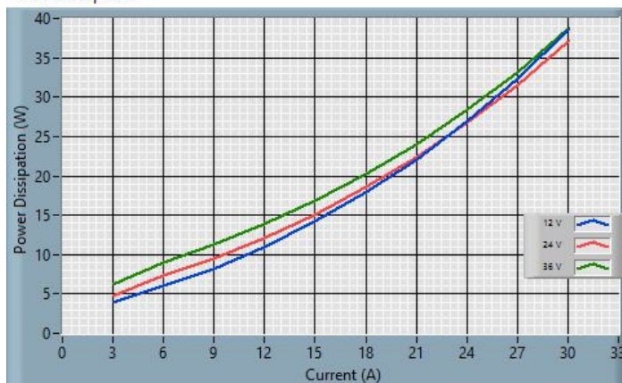
Power Dissipation
