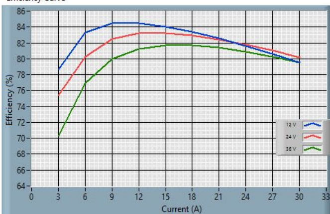
Efficiency Curve
