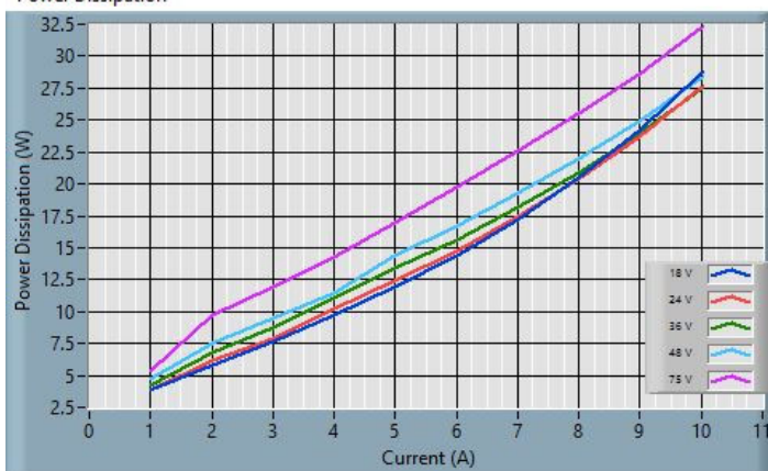
Power Dissipation
