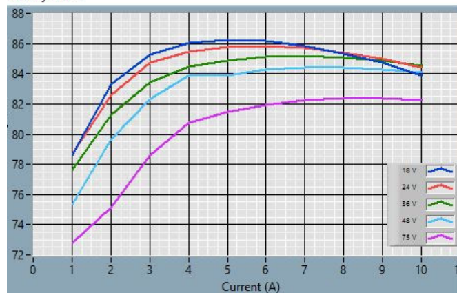
Efficiency Curve
