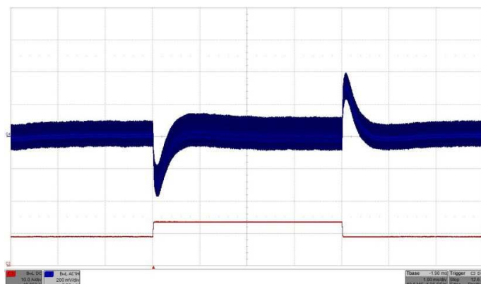
Fig. 30: Output voltage response to load current step change 50% - 75% - 50% (9A - 13.5A - 9A) with di/dt = 1A/\mu s at V_{IN} = 24V . Top trace (C4): Output voltage (200 mV/div.). Bottom trace (C3): Load current (10A/div.). C_O 470 \mu F /70m \Omega . Time: 1ms/div.
