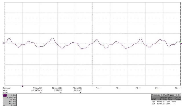
Fig. 21: Input reflected ripple current, i_c (500 mV/mV), measured at input terminals at full rated load current at V_{IN} = 24V . Refer to Fig. 2 for test setup. Time: 2 \mu s/div. RMS input ripple current is 1.235 \times 500mA = 617.5mA .
