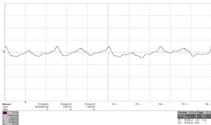
Fig. 33: Input reflected ripple current, i_c (500 mA/mV), measured at input terminals at full rated load current at V_{IN} = 24V . Refer to Fig. 2 for test setup. Time: 2 \mu s /div. RMS input ripple current is 1.098 \times 500mA = 549mA .
