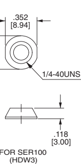
DRESS NUT
