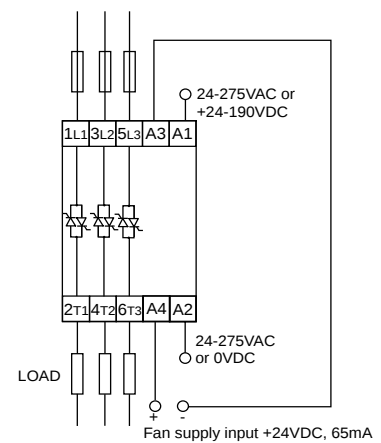
AC Control Input + fan + over-temperature protection Example: RJ3A22A32EP
