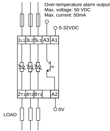
DC Control Input + over-temperature protection Example: RJ3A60D20EP
