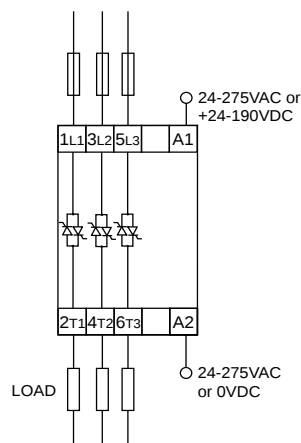
AC Control Input Example: RJ3A22A20E
