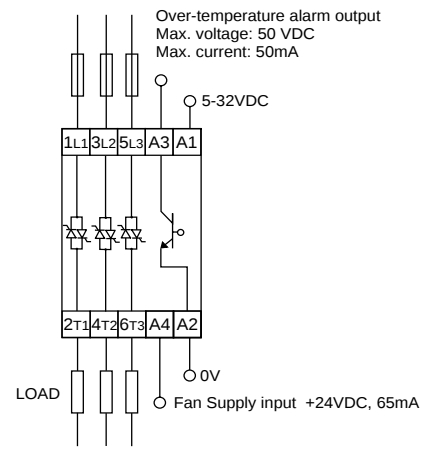
DC Control Input + Fan + over-temperature protection Example: RJ3A60D32EP
