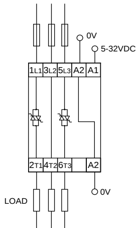
DC Control Input Example: RJ2A60D25
