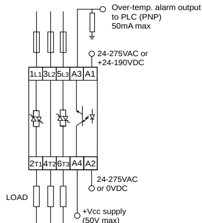
AC Control Input + over-temperature protection Example: RJ2A22A25EP
