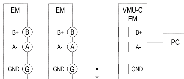
Fig. 2 RS485 COM2 to energy meters
