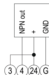
Fig. 13 NPN impulse input (product code: 2TIW)
