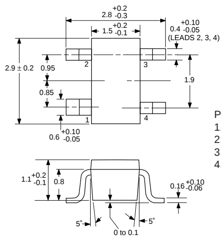
PACKAGE OUTLINE 39
