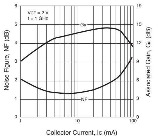
NOISE FIGURE and ASSOCIATED GAIN vs. COLLECTOR CURRENT
