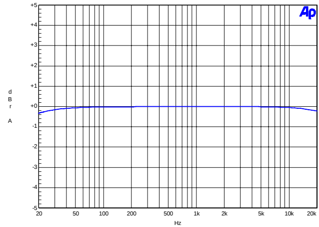
Figure 28. 192 kHz, Frequency Response
