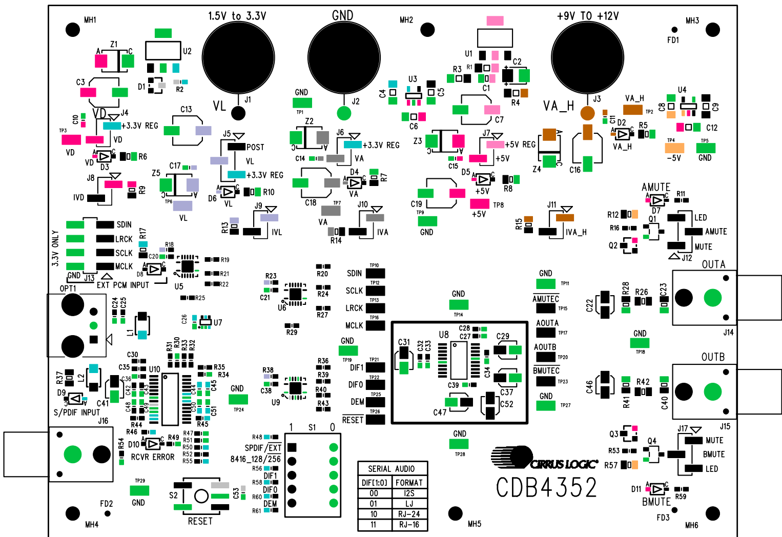
Figure 37. Silkscreen Top
