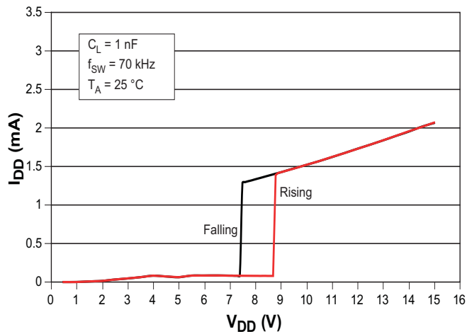
Figure 1. UVLO Characteristics
