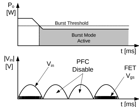
Figure 14. Burst Modes
