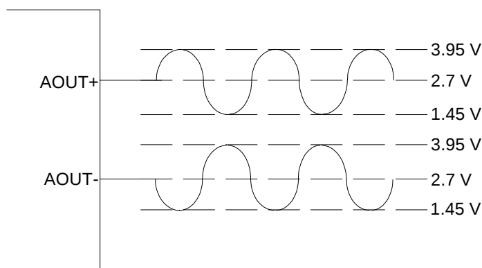
Figure 8. Full-Scale Output
