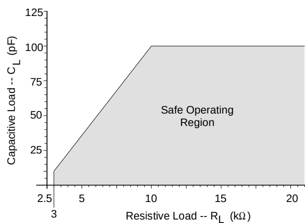
Figure 4. Maximum Loading
