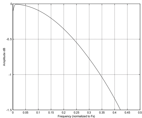
Figure 45. QSM Passband Ripple
