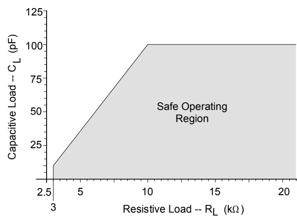
Figure 4. Maximum Loading
