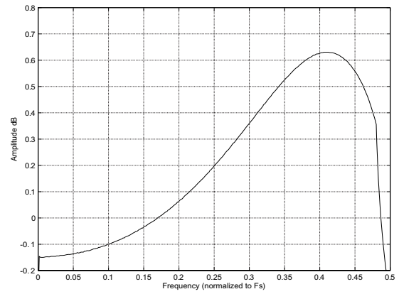
Figure 51. DSM Passband Ripple
