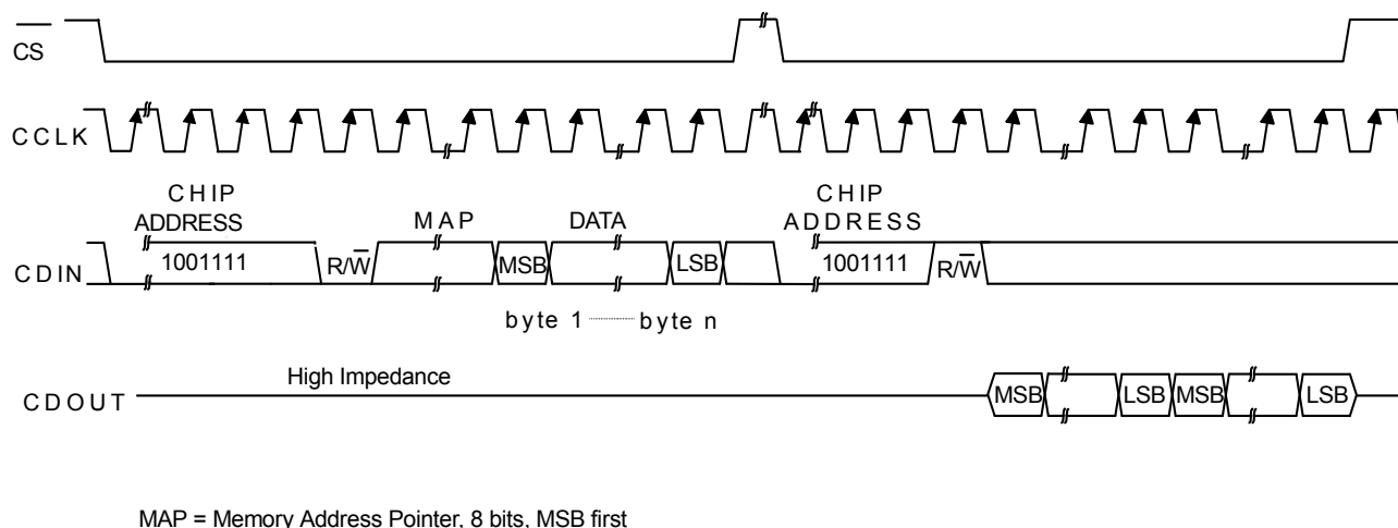
Figure 17. Control Port Timing in SPI Mode
