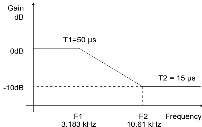
Figure 15. De-Emphasis Curve
