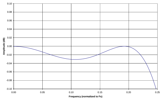
Figure 45. Quad-Speed Mode Passband Ripple
