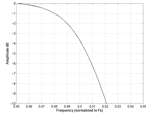
Figure 37. ADC Transition Band Detail
