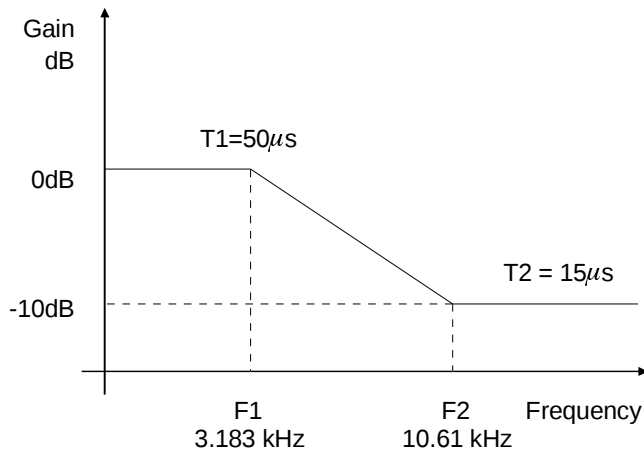
Figure 3. De-Emphasis Curve ( F_s = 44.1\text{kHz} )
