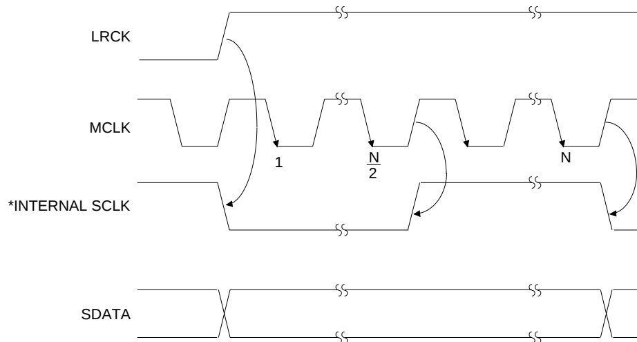
Internal Serial Clock Generation
