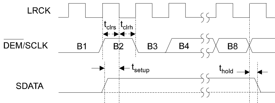
Figure 22. Configuration Timing
