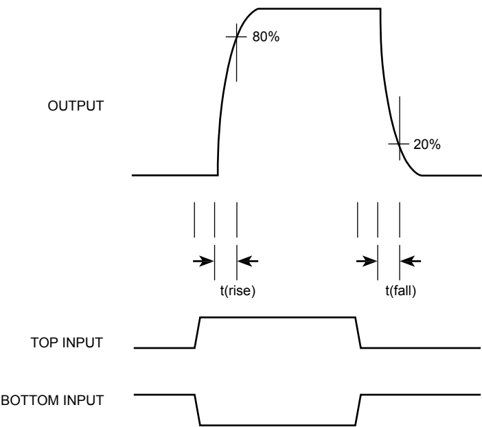
Figure 11. Output Response
