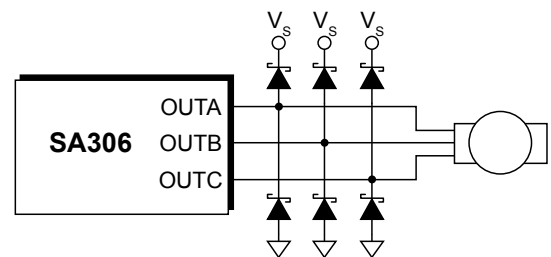
Figure 9. Schottky Diodes
