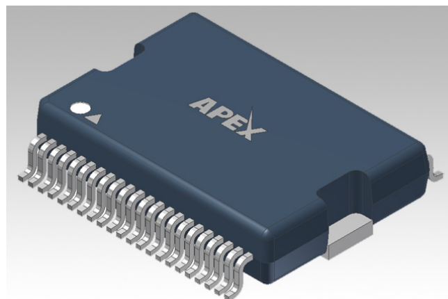
Figure 2B. 44-Pin HSOP Slug-Down, Package Style HR
